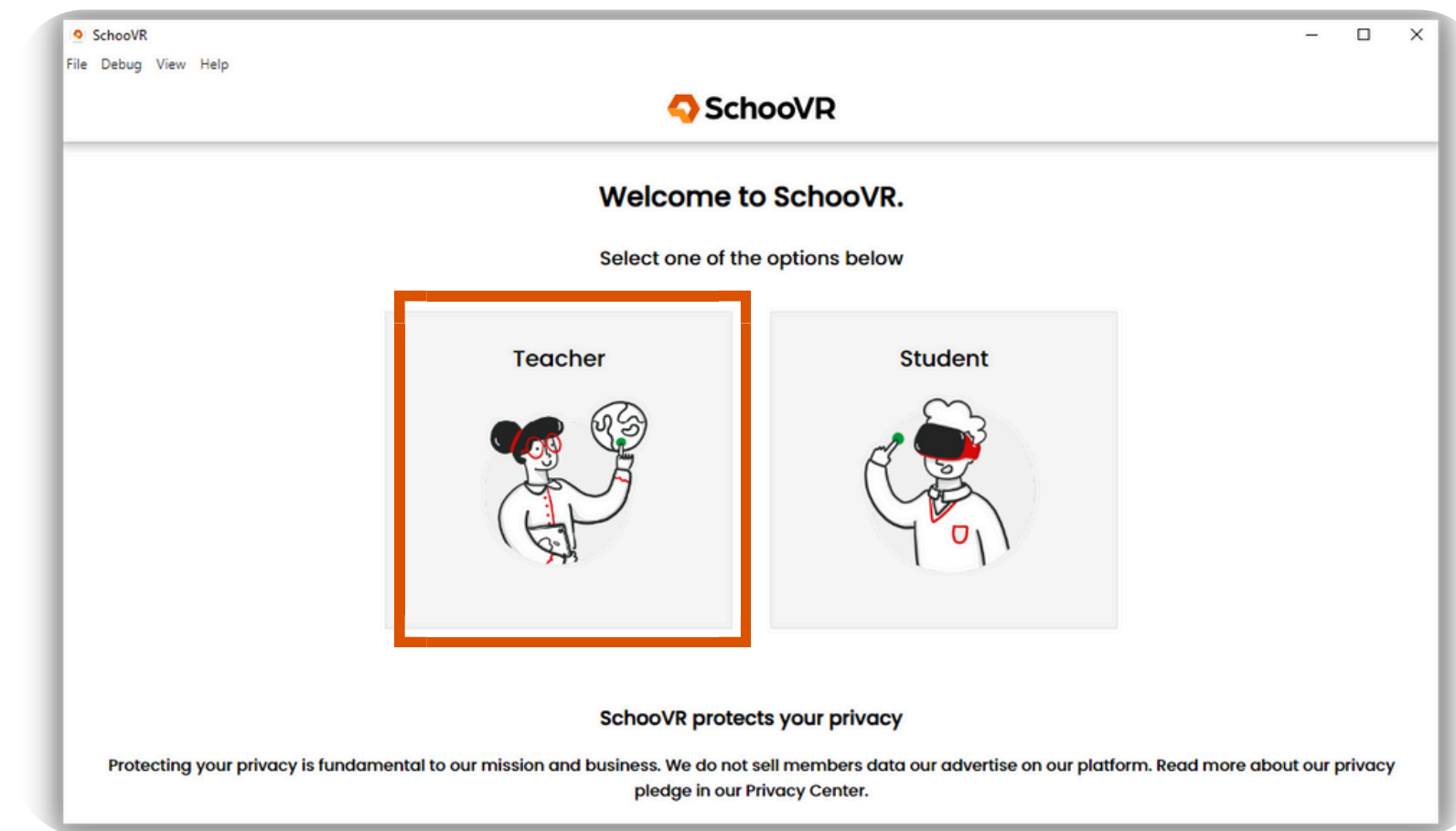
SchooVR Software
